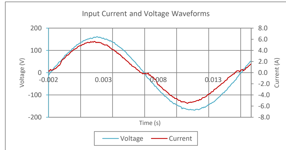
Input AC Current Waveform (ITHD = 9.96%, 50% Load)
