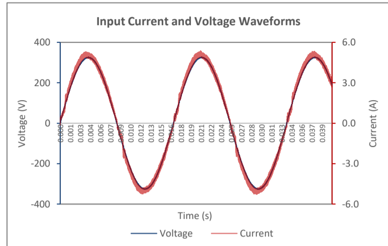
Input AC Current Waveform (ITHD = 3.16%, 50% Load)
