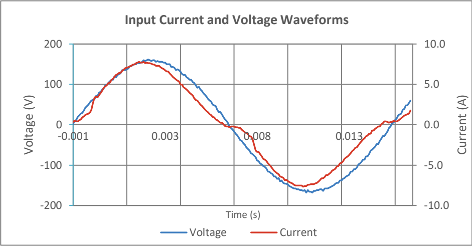
Input AC Current Waveform (ITHD = 14.88%, 50% Load)
