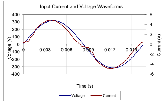
Input AC Current Waveform (ITHD = 12.93%, 50% Load)
