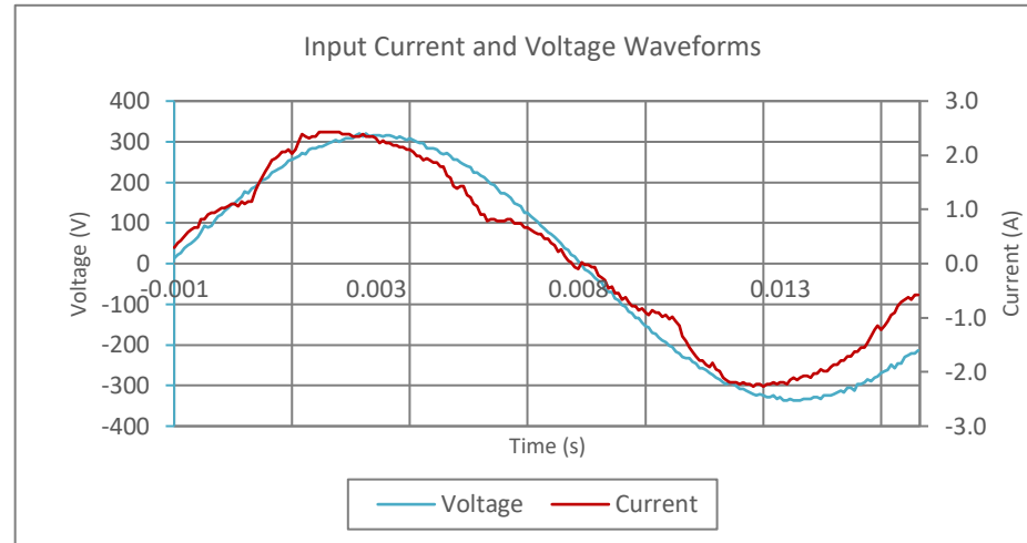
Input AC Current Waveform (ITHD = 13.71%, 50% Load)
