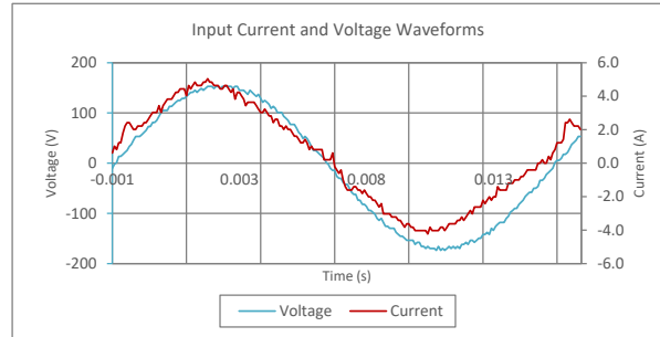
Input AC Current Waveform (ITHD = 8.45%, 50% Load)
