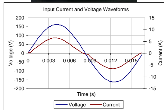
Input AC Current Waveform (ITHD = 13.81%, 50% Load)
