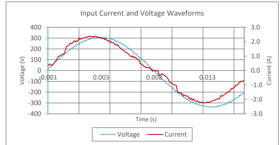
Input AC Current Waveform (ITHD = 12.4%, 50% Load)
