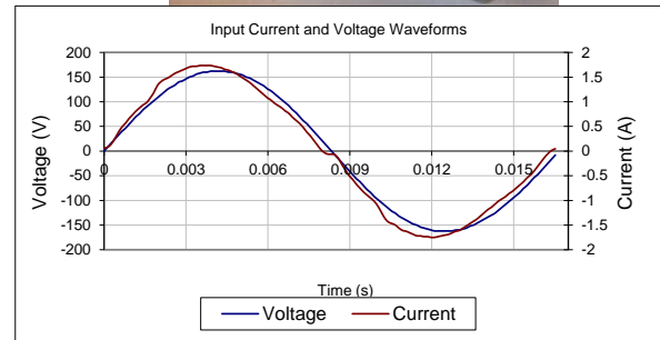
Input AC Current Waveform (ITHD = 6.56%, 50% Load)
