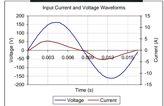
Input AC Current Waveform (ITHD = 23.21%, 50% Load)
