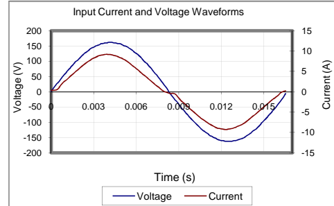
Input AC Current Waveform (ITHD = 16.88%, 50% Load)
