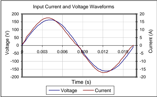
Input AC Current Waveform (THD = 8.88%, 50% Load)
