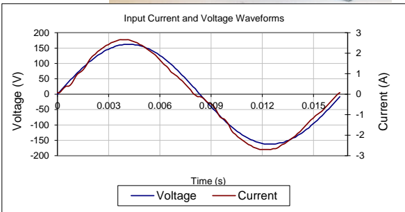
Input AC Current Waveform (ITHD = 9.23%, 50% Load)
