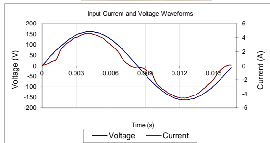
Input AC Current Waveform (ITHD = 16.86%, 50% Load)
